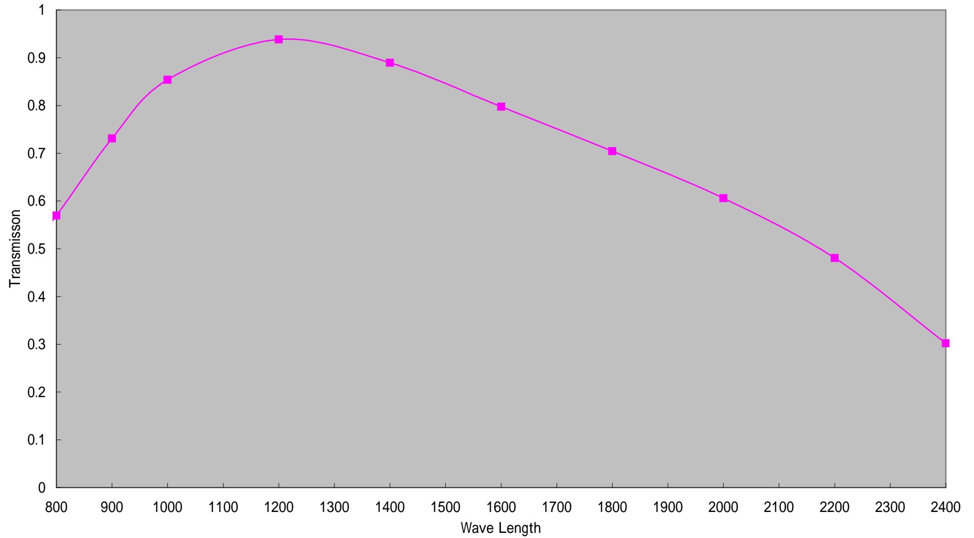
LM12HC-SW (976IR) Transmission
