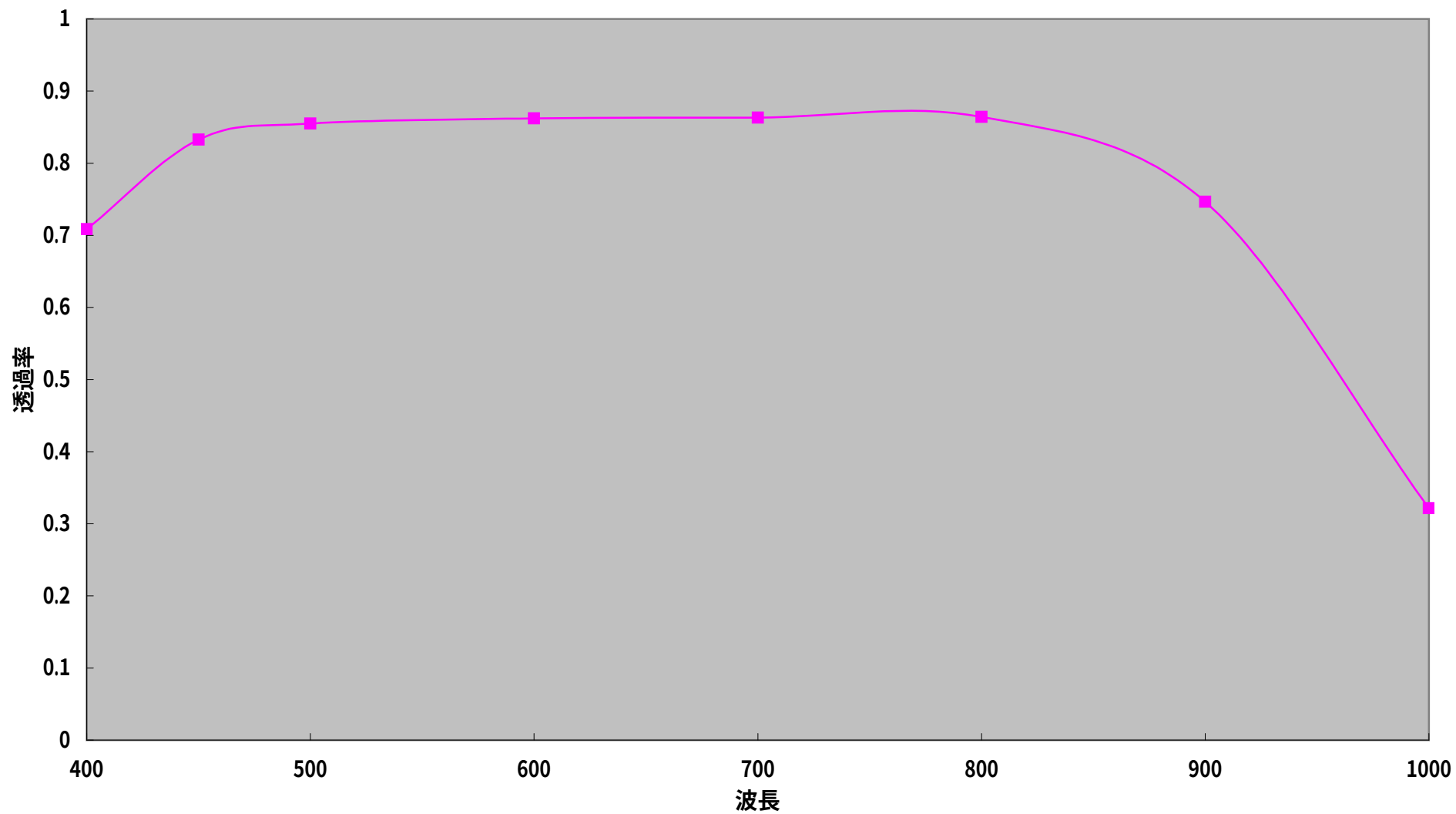
LM25JC10M 透過率
