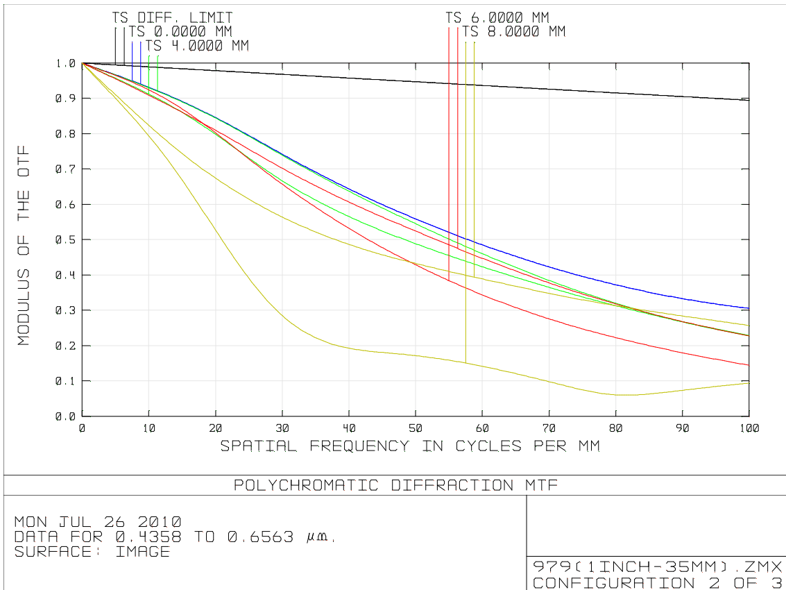
MTF (Object 1.0m)
