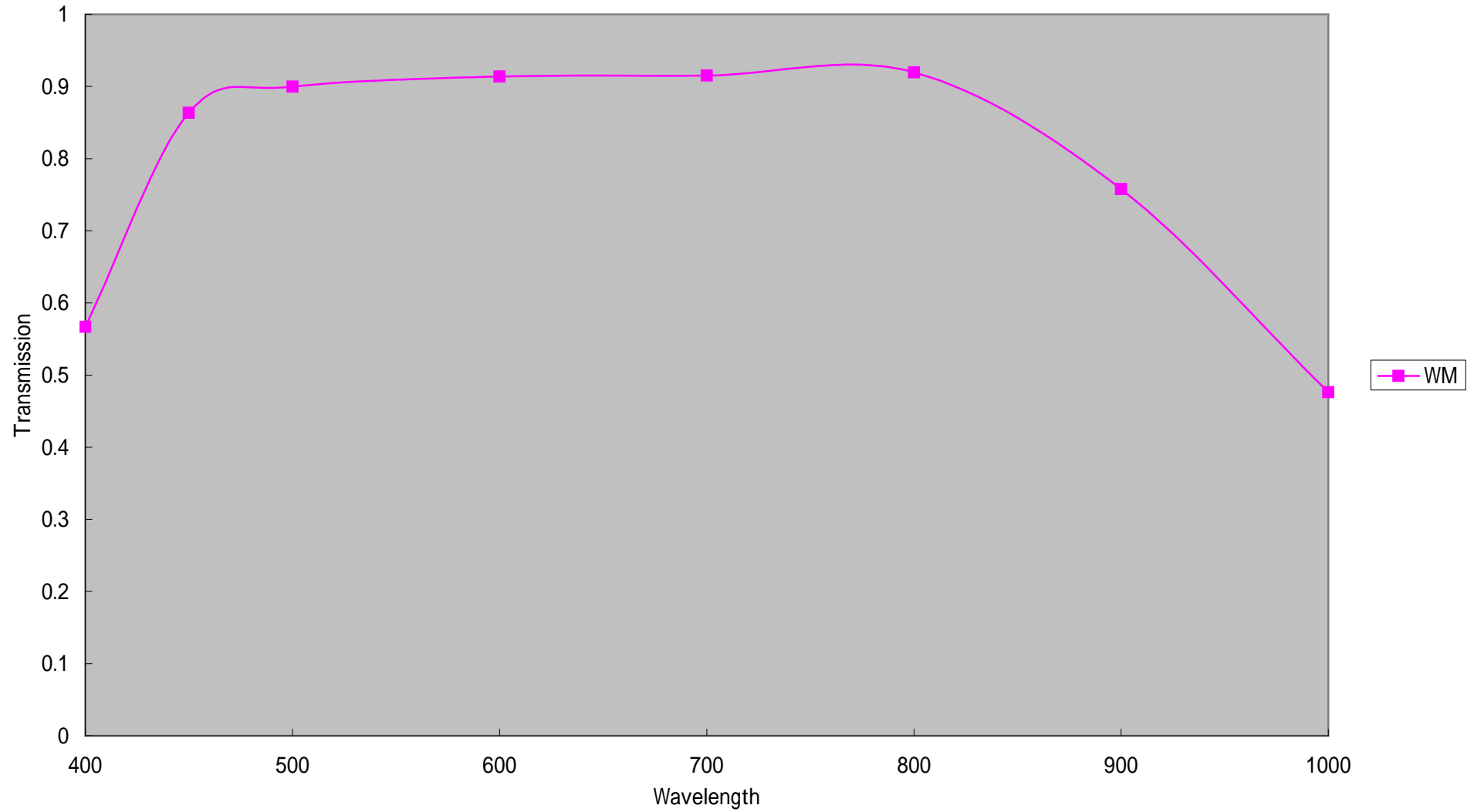
LM35XC Transmission
