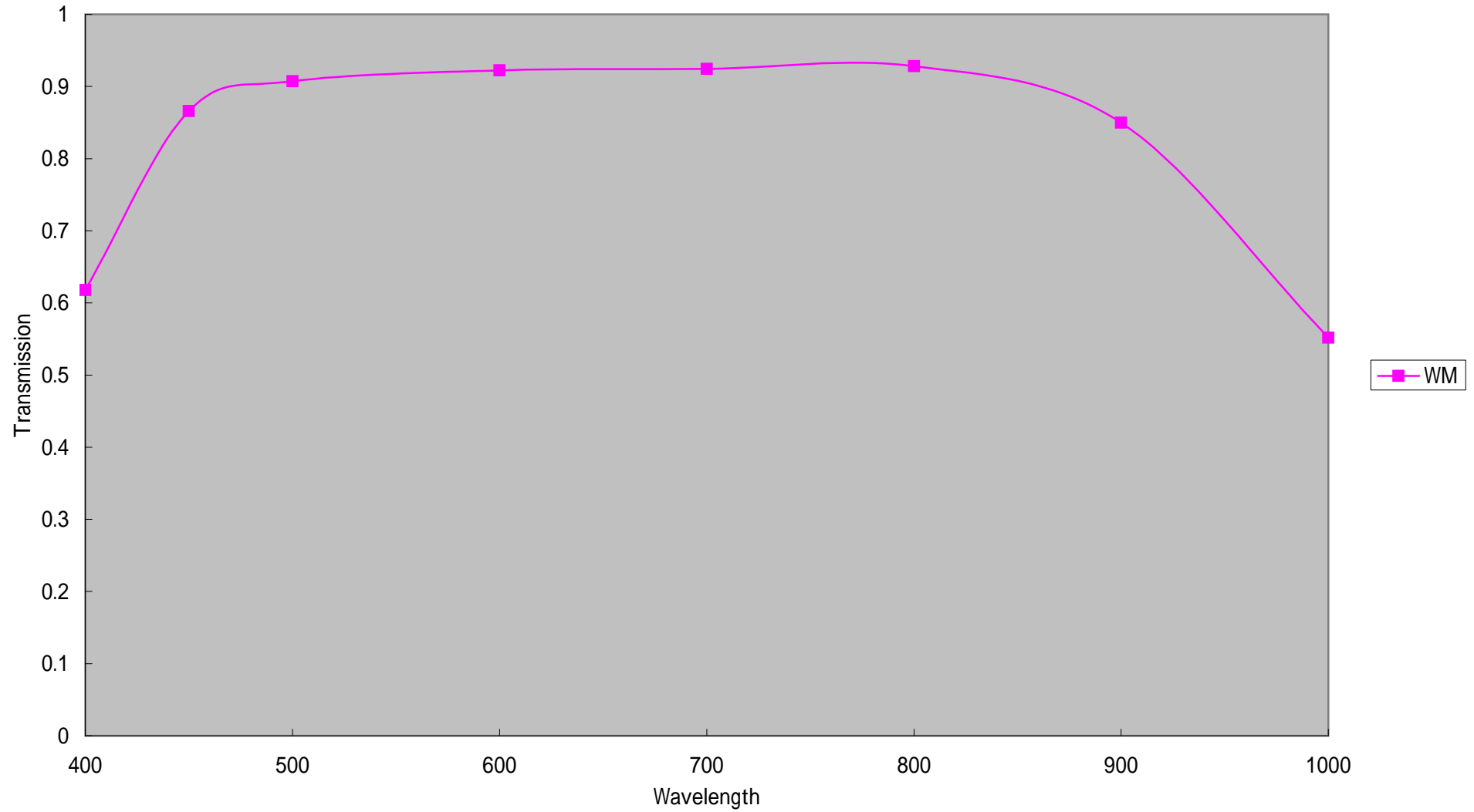
LM50-XC Transmission
