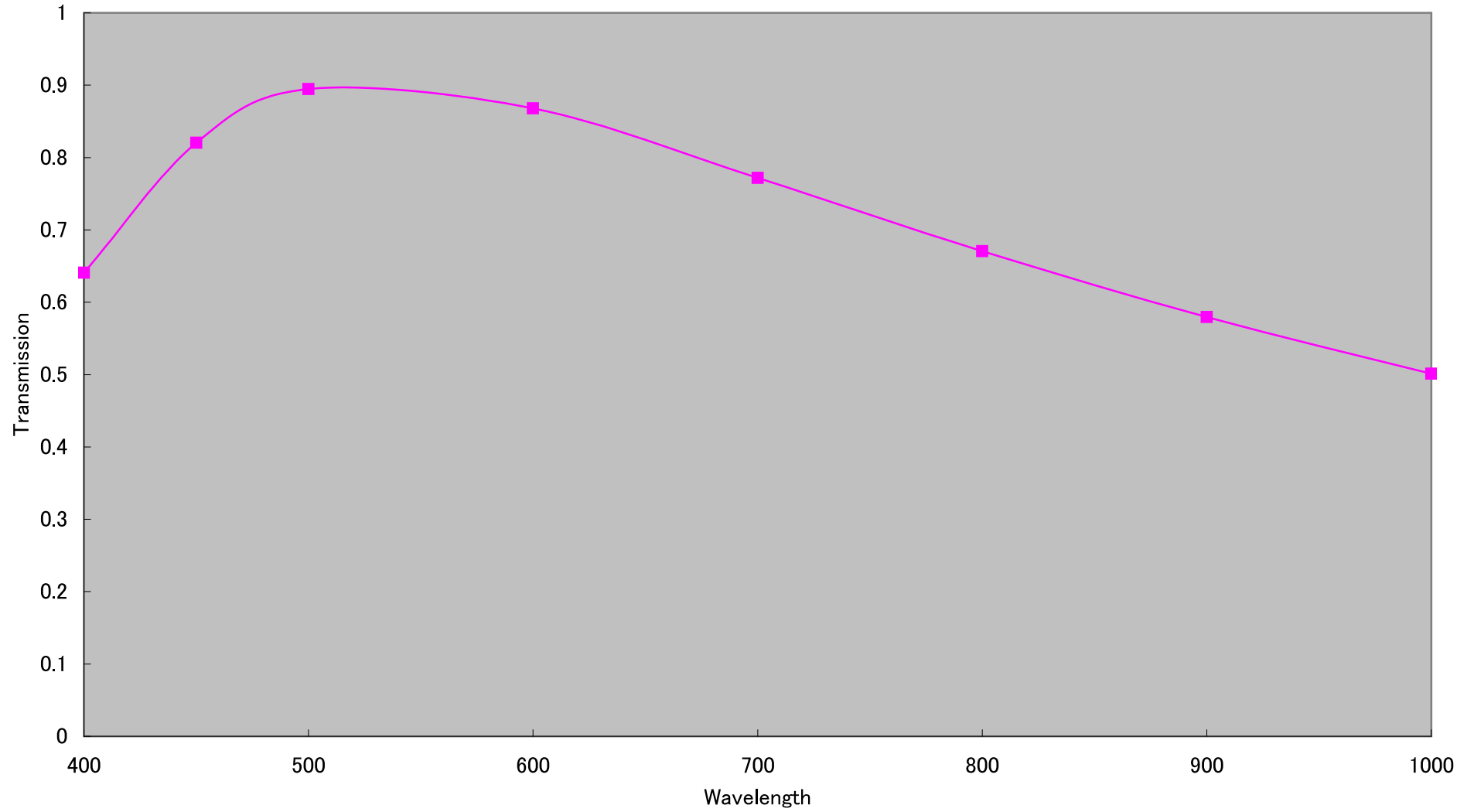
LM8JCM-V Transmission
