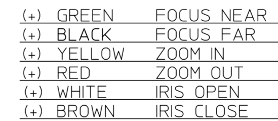
② MOTOR CABLE (FOCUS, ZOOM, IRIS)
