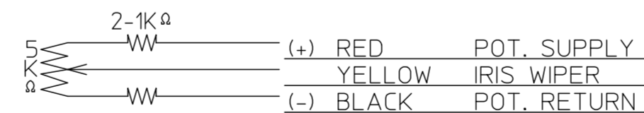
① POT. CABLE (FOCUS, ZOOM, IRIS)
