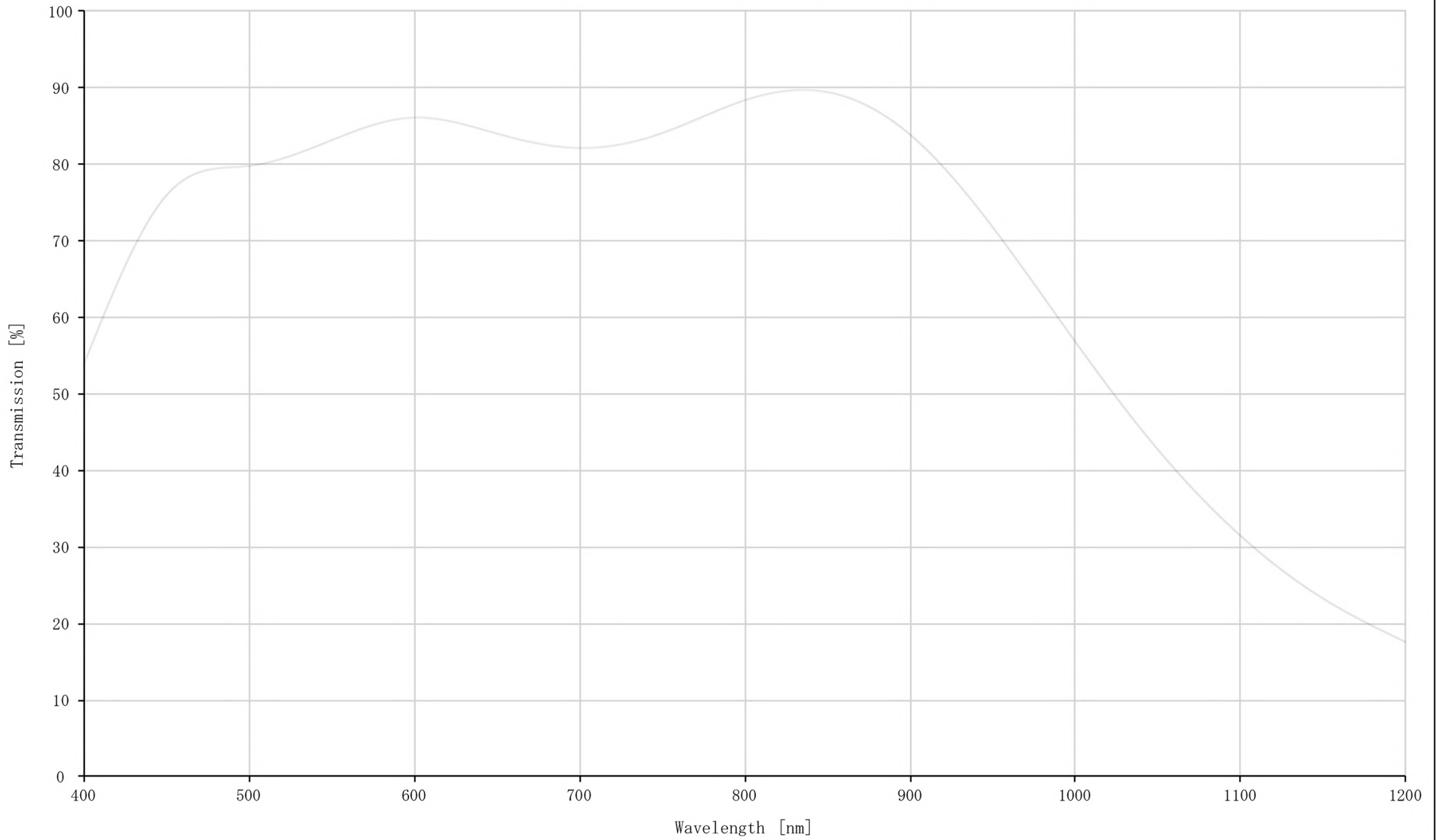
LM18VM Transmission
